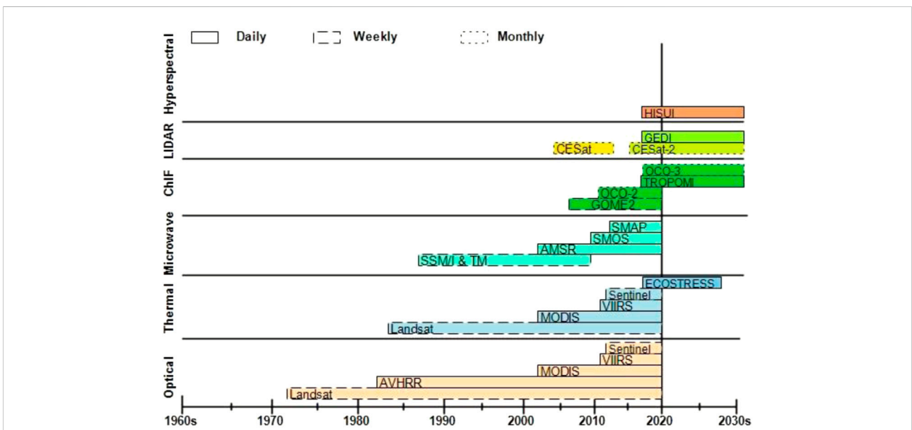
FIGURE 4 Advances in satellite imagery and multi-spectral RS of dryland vegetation dynamics. Historical milestones are provided from the 1960s to the 2030s. Timelines of LiDAR, chlorophyll fluorescence (ChIF), thermal infrared (TIR), microwave, optical, and hyperspectral earth observation satellites are shown. The progression of satellite capabilities from optical to hyperspectral indicates both the rising spatial and temporal resolution of sensor information as well as the extension of RS techniques in drylands. Modified and adapted from (Kuenzer et al., 2014; Smith et al., 2019). The color differentiates the type of satellite and its capability. The solid, semi-solid, and dash-dash lines represent daily, weekly, and monthly scales, respectively, as the data acquisition time.
