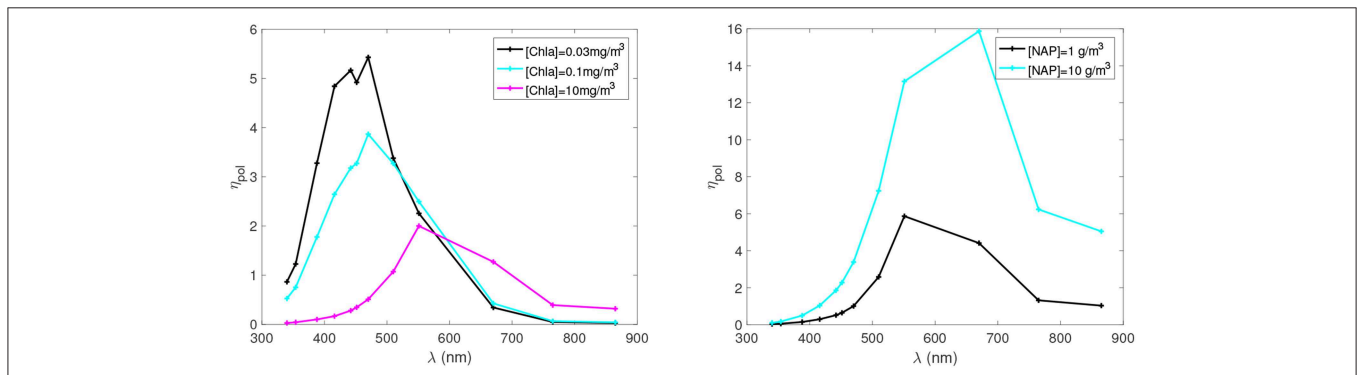
FIGURE 6 | Polarized water-leaving relative percentage contribution in the TOA polarized reflectance for the same case as Figure 4 . Reprinted with permission from Zhai et al. (2017a), The Optical Society (OSA).
