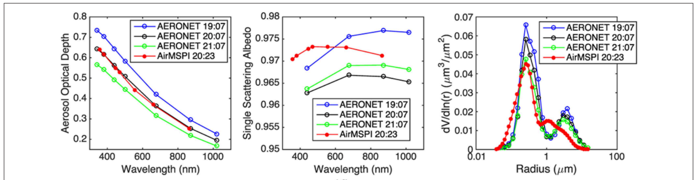
FIGURE 7 | AirMSPI-retrieved aerosol optical depth (AOD), single scattering albedo (SSA), and volume-weighted aerosol size distribution collocated with the Fresno AERONET site on January 6, 2012, compared to the AERONET-derived values. Different times of observation noted. Adapted with permission from Xu F. et al. (2017), John Wiley & Sons.
