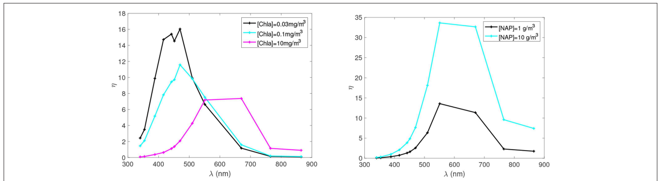
FIGURE 5 | Water-leaving relative percentage contribution in the TOA reflectance for the same case as in Figure 4 . Reprinted with permission from Zhai et al. (2017a), The Optical Society (OSA).
