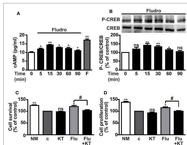
FIGURE 3 | Involvement of cAMP/PKA/CREB signaling in Fludro survival and proliferative effects. (A) Intracellular cAMP levels in growth factor-deprived AHPs cultured for the indicated times with 1 \mu\text{M} Fludro, in the presence of phosphodiesterase inhibitor IBMX (100 \mu\text{M} ), that was added 30 min before stimulation. Forskolin (F) (50 \mu\text{M} for 2 min) was used as positive control. Results are the mean \pm SE of three independent experiments (* P < 0.05, ** P < 0.01 vs. time 0). (B) CREB phosphorylation on serine 133 (top panel) evaluated by Western blot in lysates from AHPs incubated with Fludro (1 \mu\text{M} ) for the indicated times. Equal protein loading was determined by reprobing with total CREB antibody (bottom panel). Blots are representative of three independent experiments. Graphs show the densitometric analysis of phosphorylated proteins normalized to total proteins and reported as percentage of basal (* P < 0.05 and ** P < 0.01 vs. time 0; ns, not significant). (C,D) Cell survival and proliferation assessed by MTT assay and BrdU, respectively, in AHP cells cultured in normal medium (NM) or in growth factor-deprived medium (c, control medium) for 12 h, and then for further 24 h with 0.5 \mu\text{M} KT5720 (KT), either alone or with 1 \mu\text{M} Fludro (Flu). Data, expressed as percentage of control, are the mean \pm SE ( n = 3); * P < 0.05, ** P < 0.01 vs. c; # P < 0.05; ns, not significant.
