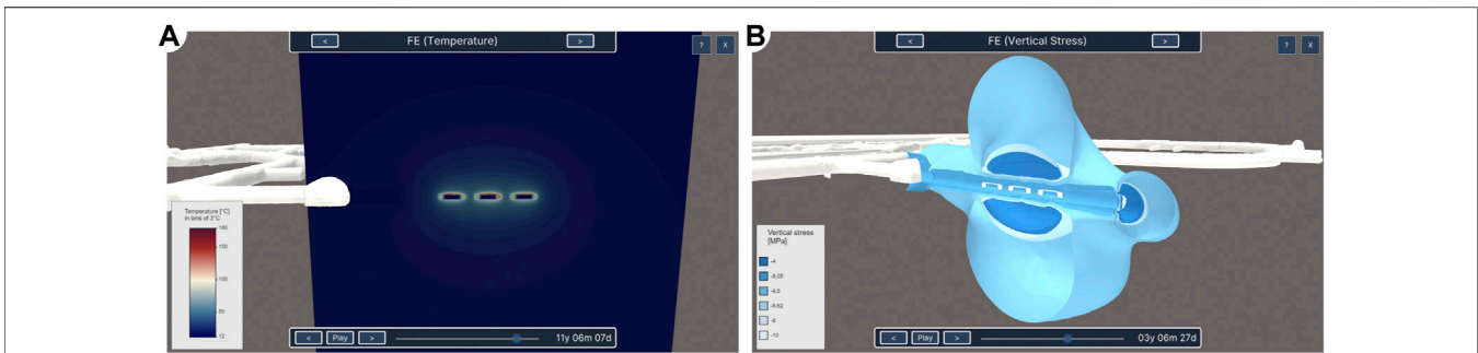
FIGURE 10 | The two visualisation techniques for simulation results in the scope of the FE experiment (A) the modelled temperature as discrete bins of 3°C on a clipped volume and (B) the modelled vertical stress as six contour surfaces.
