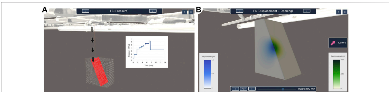
FIGURE 11 | Two visualisations of the Fault Slip Experiment (A) a general illustration of the experiment and (B) simulation results with an additional arrow indicating the change of pressure relative to the last time step.
