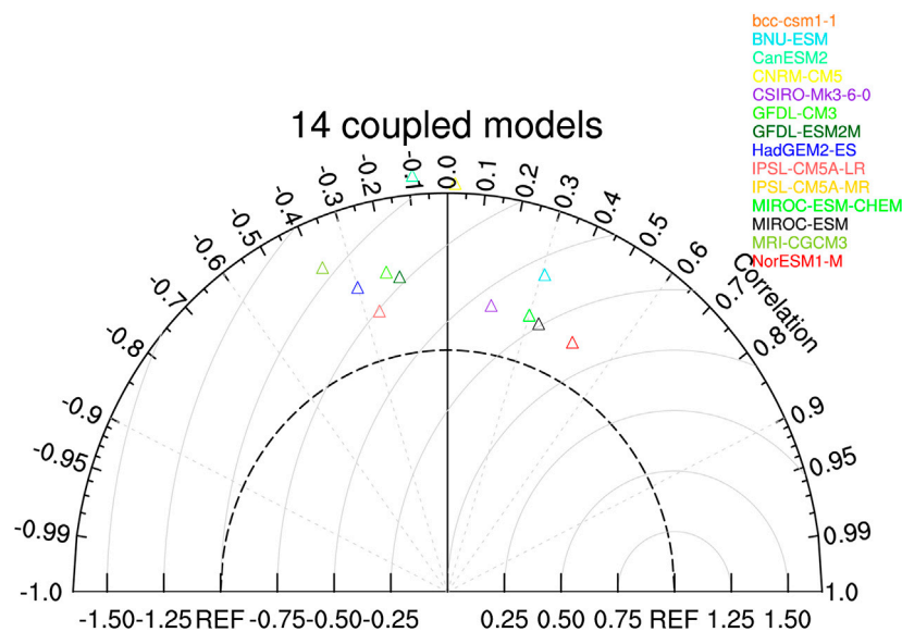
FIGURE 6 | Taylor diagram of the interannual variability of the annual mean 12-month Standardized Precipitation Evapotranspiration Index. All of the GCMs are shown, except for two global climate models (CanESM2 and CNRM-CM5) with large standard deviations.
