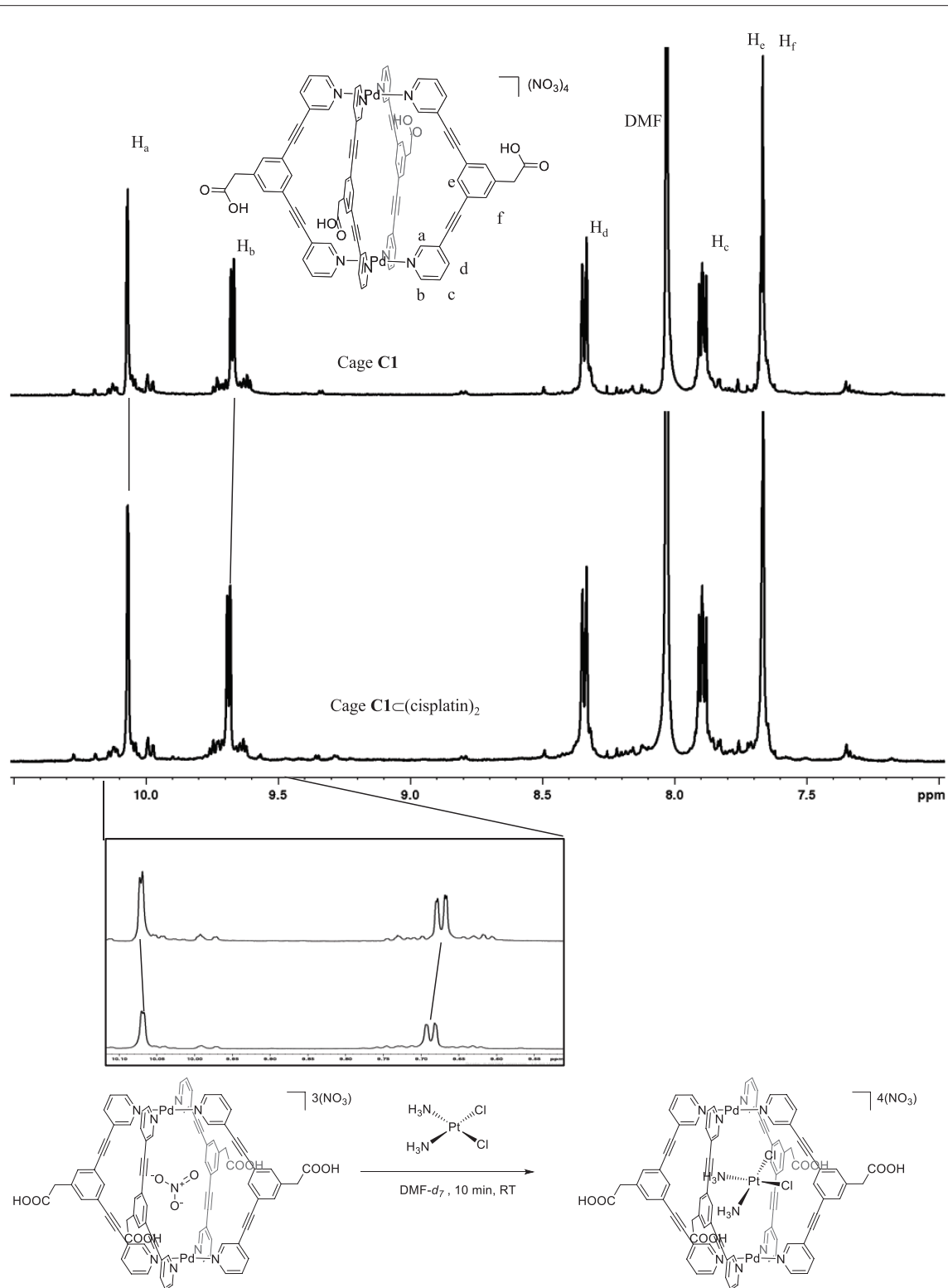
FIGURE 1 | Cisplatin encapsulation in a metallacage following displacement of nitrate ions from the cavity. Stacked spectra of cage C1 in DMF- d 7 (top) and cage C1 after the addition of 2 equivalent of cisplatin (bottom). Box : Zoom-in of signals for peaks H a and H b with chemical shifts of \delta = -0.002 ppm (upfield) and +0.01 ppm (downfield), respectively.
