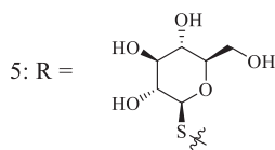
SCHEME 1 | Top: General scheme for [\text{Pd}_2\text{L}_4]^{4+} metallacage formation via self-assembly. Bottom: Numbered (n) chemical structures of the exo -functionalized groups envisioned to improve the cages' aqueous solubility.
