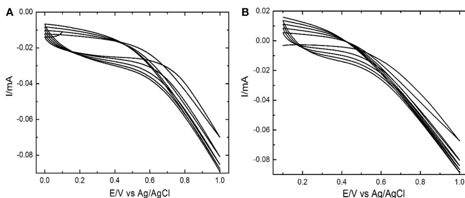
FIGURE 1 | Cyclic voltammogram during electrochemical deposition of unmodified (A) Ppy and (B) Ppy/SWNTs nanocomposite at a scan rate of 50 \text{ mV s}^{-1} .
