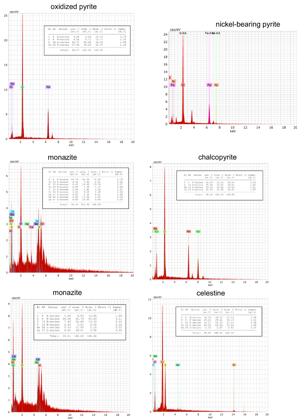
Figure S1. EDS Spectra for Figure 11.
