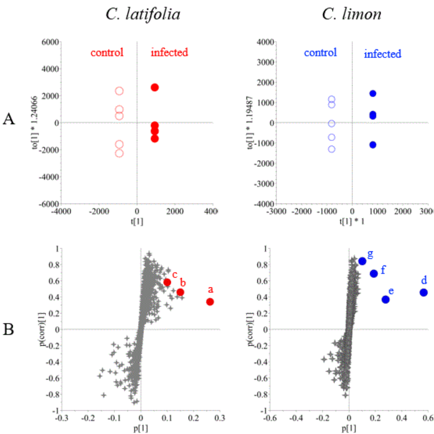
Supplementary Figure S2| (A) OPLS-DA and (B) Loading scores of C. lemon (S) x C. latifolia (R), based on LC-MS/MS 60 days analysis.
