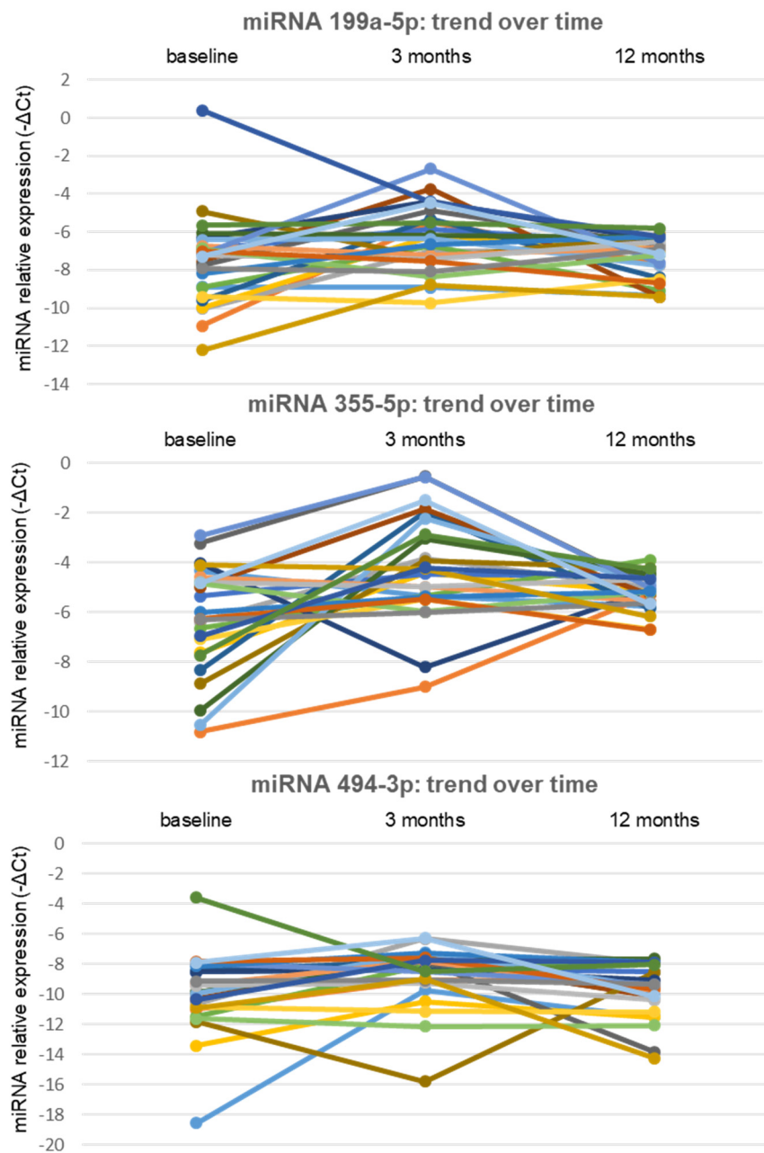
Figure S1. miRNA trend over time. MiRNA levels were measured in serum samples from 25 prepubertal patients with IIGHD and are expressed as -\Delta Ct where \Delta Ct is calculated as: Ct\ miRNA - Ct\ miR-16-5p
