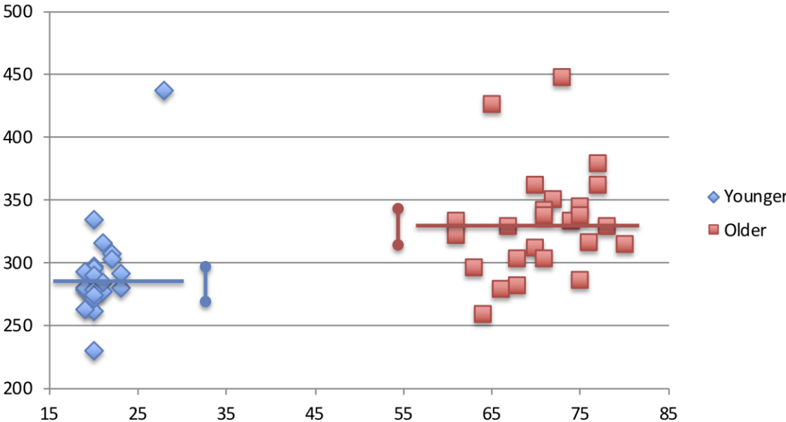
Supplementary Figure 1. Mean RTs on the X-test for each participant. Average RTs are indicated with horizontal lines. Vertical lines indicate group means plus or minus one standard error.
