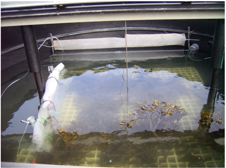
Fig. S1 Benthic mesocosm facility on the island of Sylt (List, Germany). (A) One of the 12 mesocosms with opened lid. (B) View inside one mesocosms onto the vertically adjustable grating populated with 11 individuals of Fucus mytili .
