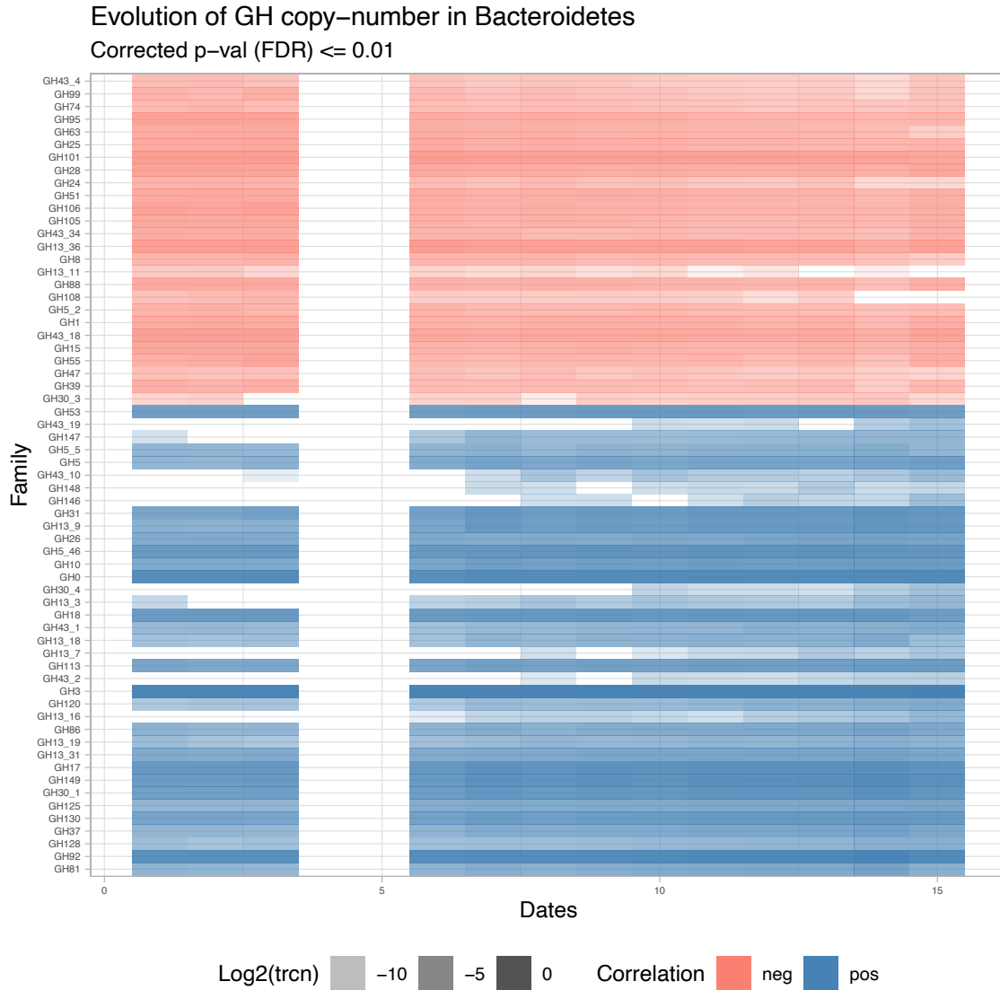
Supplementary figure 5. Heatmap showing the copy number of GH families (trcn, log 2 scale) across the time series. Only families showing a significant (corrected p-val ≤ 0.01) correlation with chlorophyll A are shown. Families are ordered by their correlation index, positive (bottom) to negative (top).
