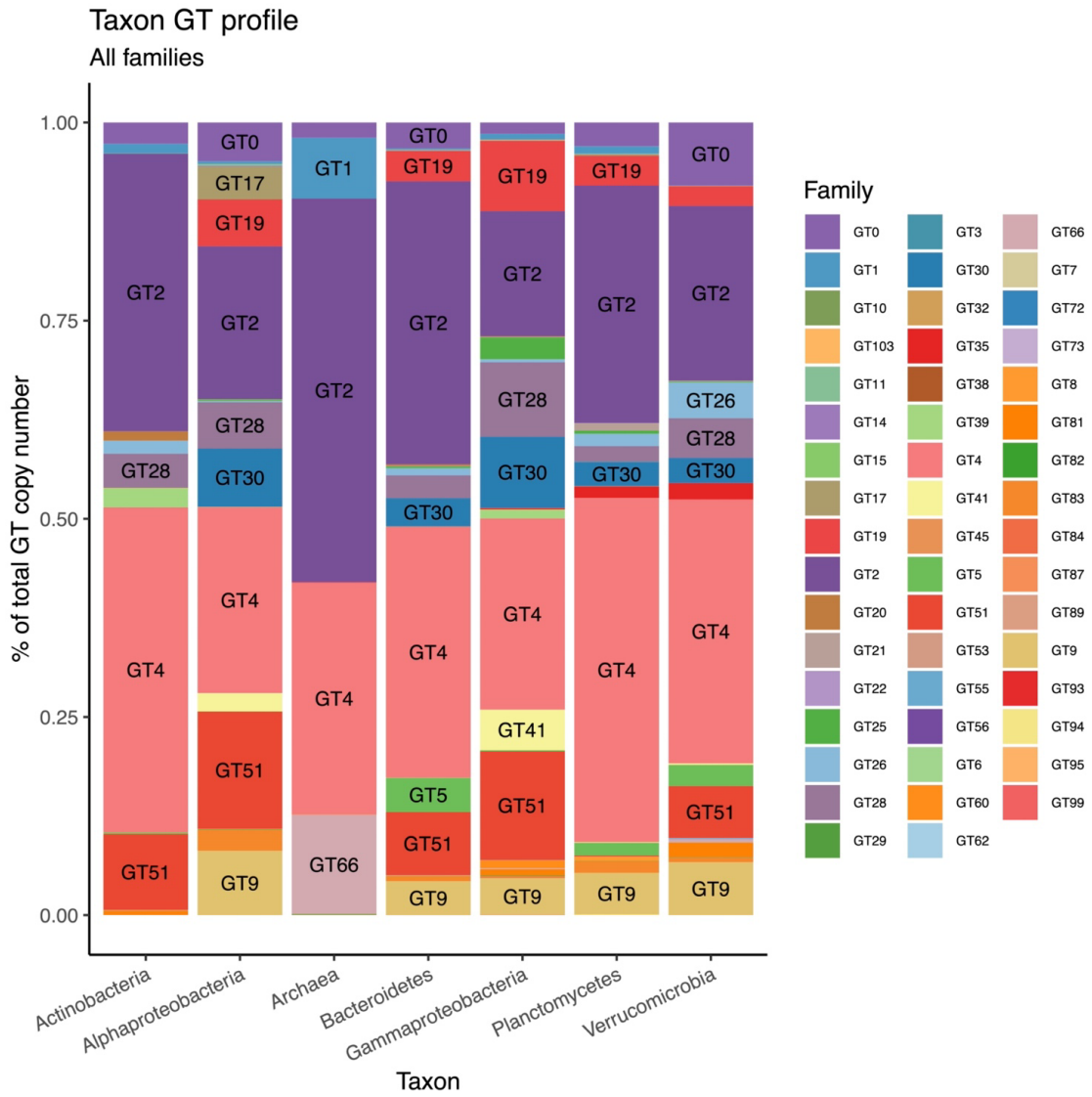
Supplementary figure 2. Glycosyl transferase (GT) profiles of different taxa, showing the percentage that each family represents out of the total copy number.
