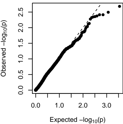
MEfloralwhite (1-dom-ref)
