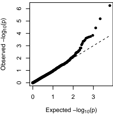
MEmediumpurple3 (additive)
