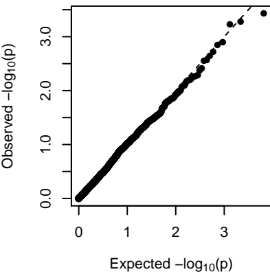
MEred (additive)
