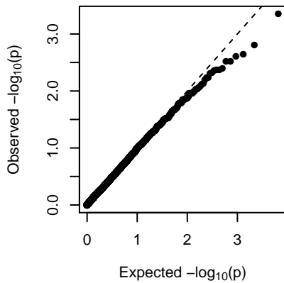
MEbrown (general)
