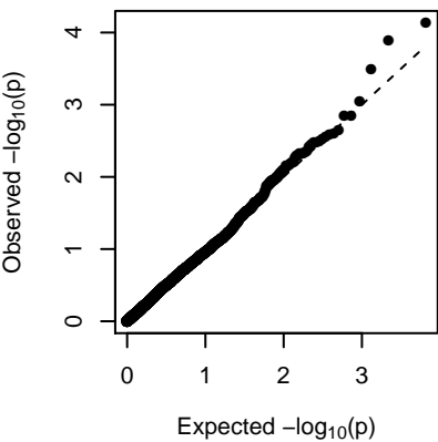
MEfloralwhite (additive)
