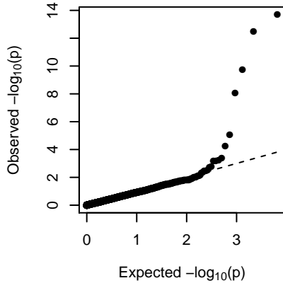
MEblue (general)
