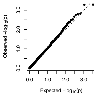
MEthistle2 (1-dom-alt)
