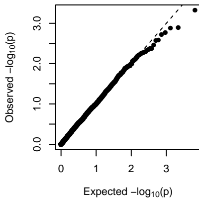
MEdarkgrey (general)
