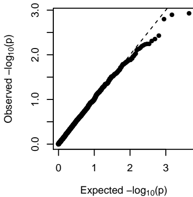
MEivory (2-dom-alt)
