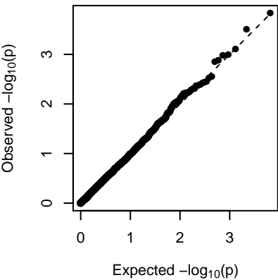
MEtan (additive)
