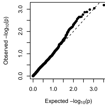
MEblack (1-dom-alt)
