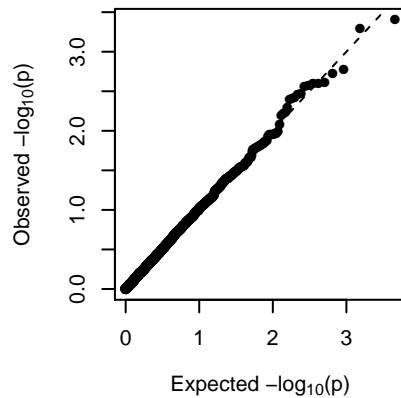
MElightyellow (2-dom-ref)
