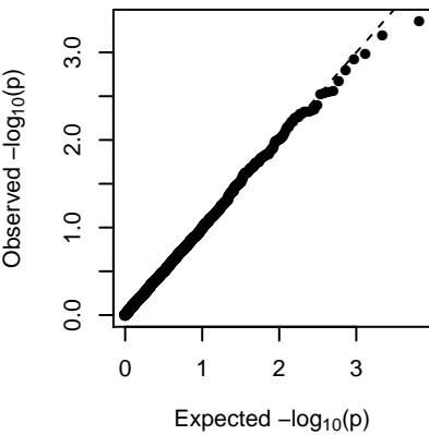
MEcyan (additive)
