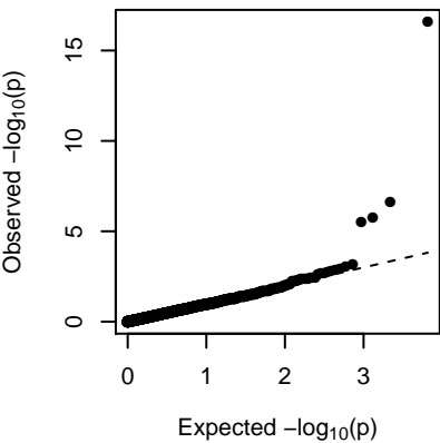
MEthistle1 (additive)
