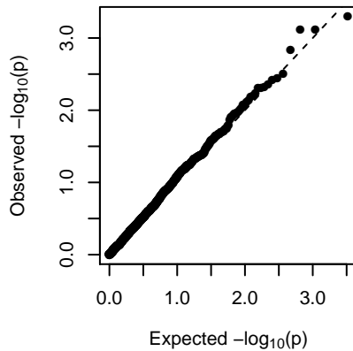
MEplum1 (1-dom-alt)
