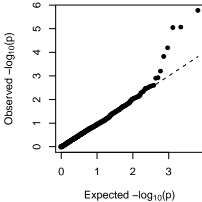
MEdarkorange2 (general)
