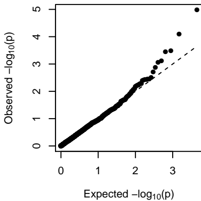
MEtan (2-dom-alt)
