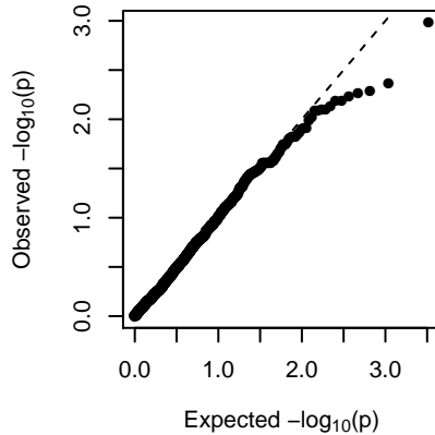
MEdarkgreen (1-dom-alt)
