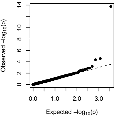
MEthistle1 (1-dom-ref)
