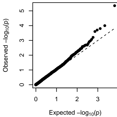
MEred (general)
