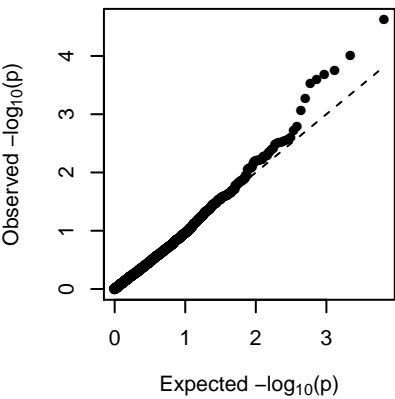
MEroyalblue (additive)
