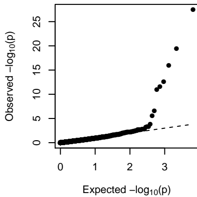
MEdarkorange (general)
