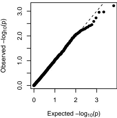
MEivory (additive)
