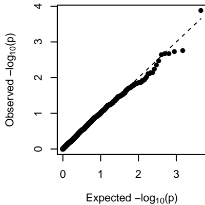
MEskyblue3 (2-dom-alt)
