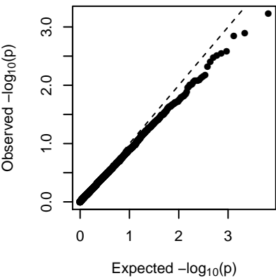
MEdarkmagenta (additive)
