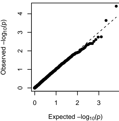
MEskyblue3 (additive)
