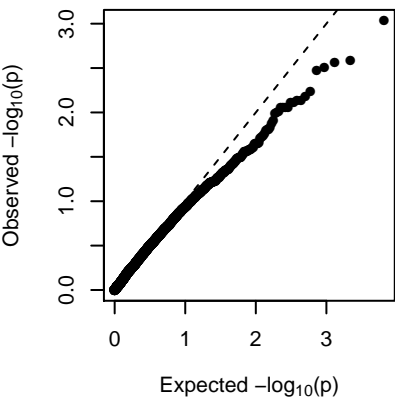
MEdarkgreen (additive)
