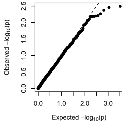
MEdarkslateblue (1-dom-alt)
