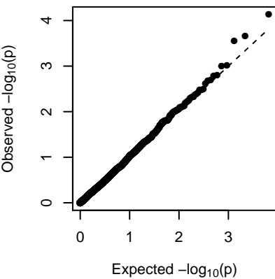
MEbrown4 (additive)
