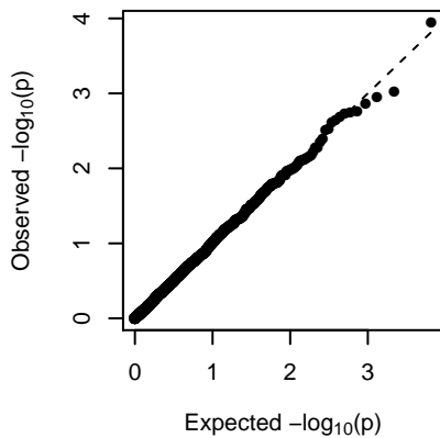
MEskyblue3 (general)
