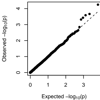
MEtan (general)
