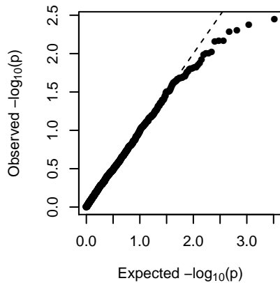
MEyellowgreen (1-dom-alt)
