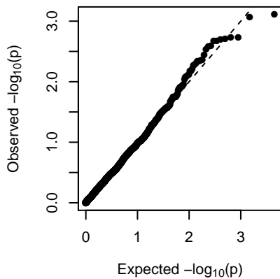
MEfloralwhite (2-dom-alt)
