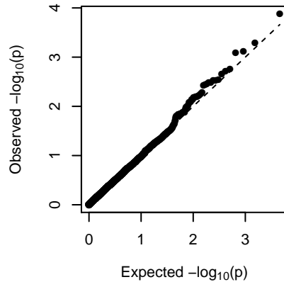
MEbisque4 (2-dom-ref)
