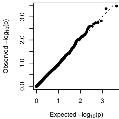
MEroyalblue (2-dom-alt)
