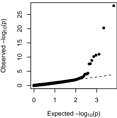
MEdarkorange (additive)
