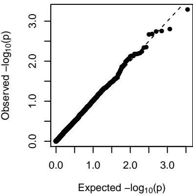
MEthistle2 (1-dom-ref)
