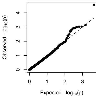
MEyellowgreen (2-dom-alt)
