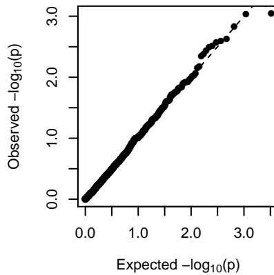
MEivory (1-dom-alt)
