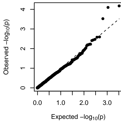
MEturquoise (1-dom-alt)
