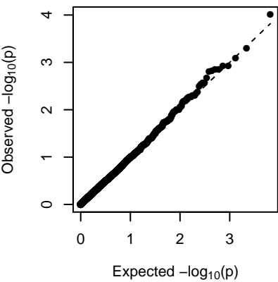
MEorangered4 (additive)
