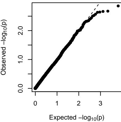
MEbrown (additive)
