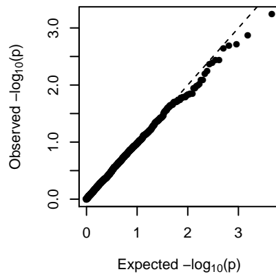
MEskyblue3 (2-dom-ref)
