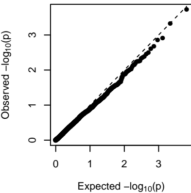
MEturquoise (additive)
