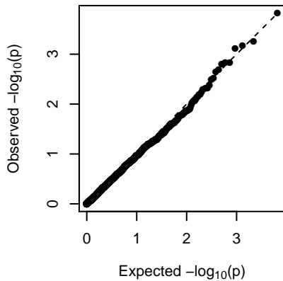
MEplum1 (general)
