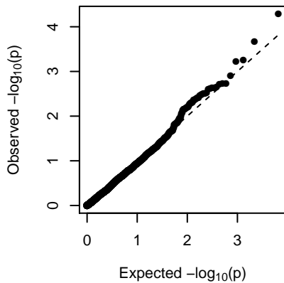
MEyellowgreen (general)
