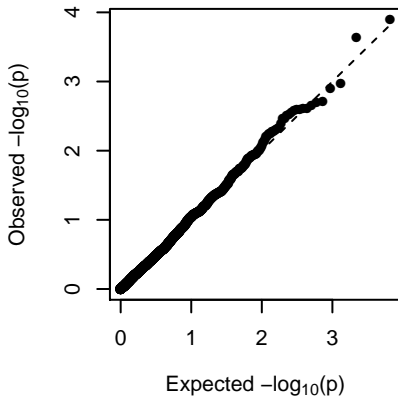
MEyellow (general)
