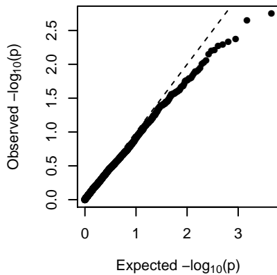
MEturquoise (2-dom-alt)
