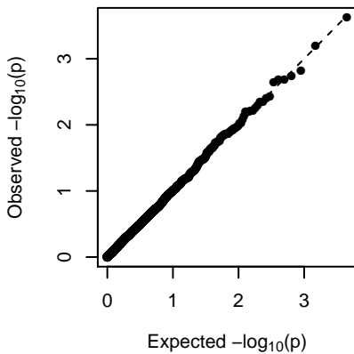
MEyellow (2-dom-alt)
