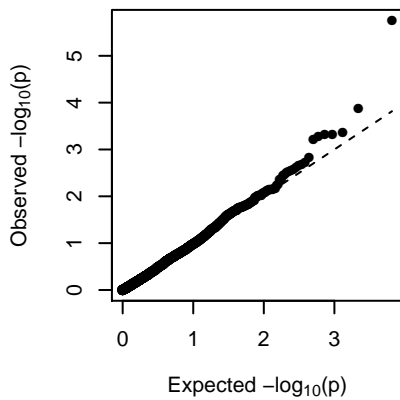
MEdarkslateblue (general)
