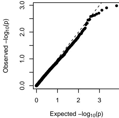
MEturquoise (general)
