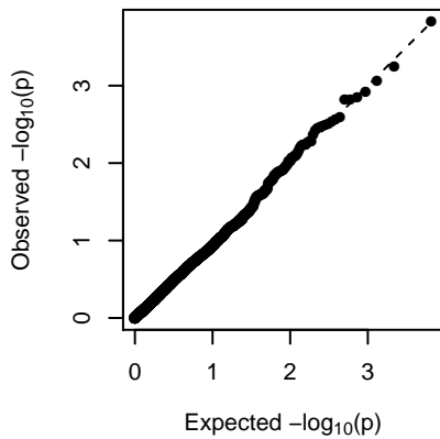
MEdarkred (general)
