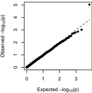
MEgrey (additive)
