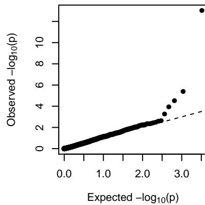
MEbisque4 (1-dom-alt)
