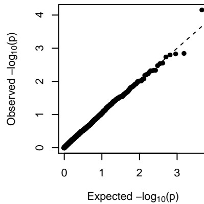
MEred (2-dom-ref)
