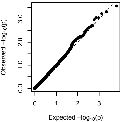
MEthistle2 (additive)
