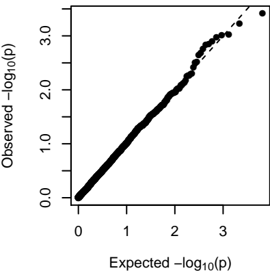
MEyellow (additive)
