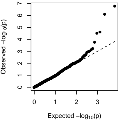
MEdarkorange2 (additive)
