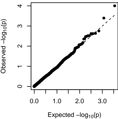
MEyellow (1-dom-ref)
