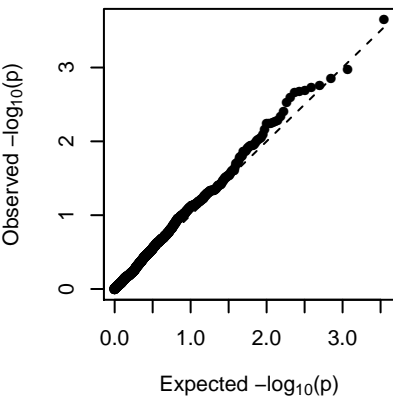
MEred (1-dom-ref)
