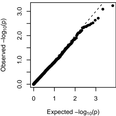
MEyellowgreen (additive)
