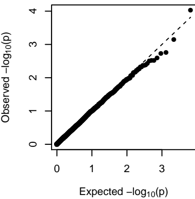
MEdarkgrey (additive)
