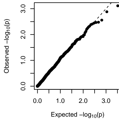
MEred (1-dom-alt)
