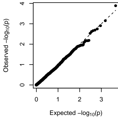
MEyellowgreen (2-dom-ref)
