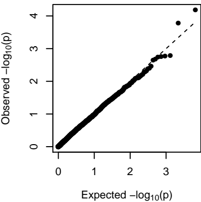
MElightyellow (additive)
