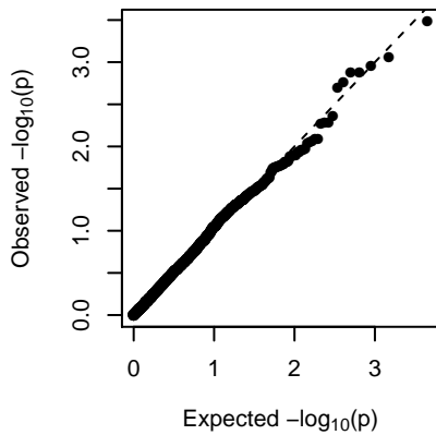
MEbrown (2-dom-alt)
