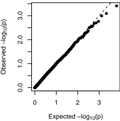
MElightgreen (additive)
