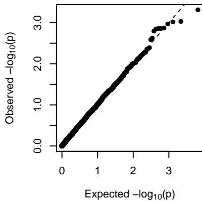
MElightyellow (general)
