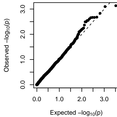
MEbrown (1-dom-alt)
