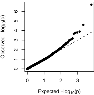
MEsienna3 (additive)
