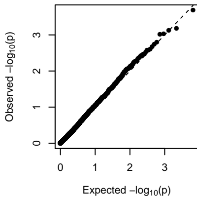
MEbrown4 (general)
