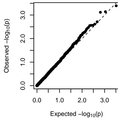
MElightsteelblue1 (1-dom-alt)
