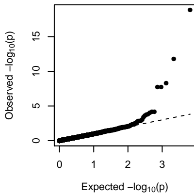
MEdarkturquoise (general)
