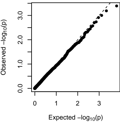
MEdarkred (additive)
