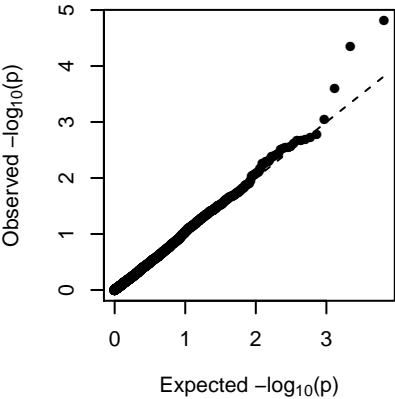
MEgreenyellow (additive)
