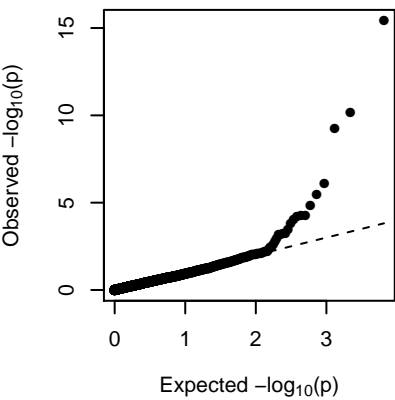
MEdarkturquoise (additive)
