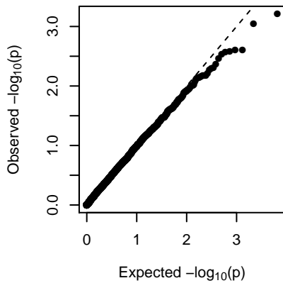
MEpink (general)
