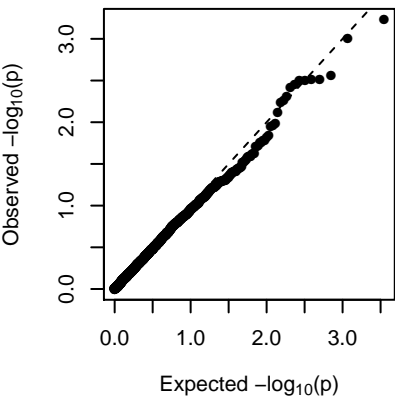
MEyellowgreen (1-dom-ref)
