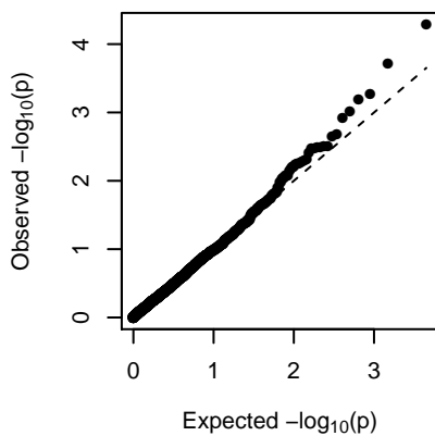
MEthistle1 (2-dom-alt)
