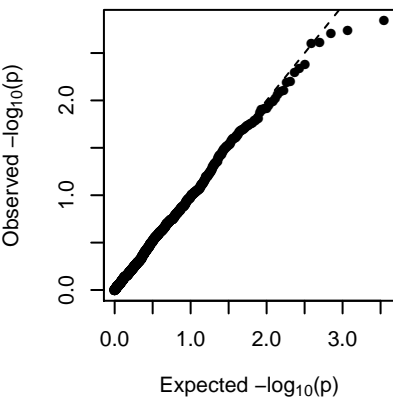
MEskyblue3 (1-dom-ref)
