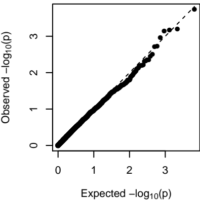
MEMagenta (additive)
