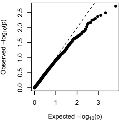
MEdarkslateblue (additive)
