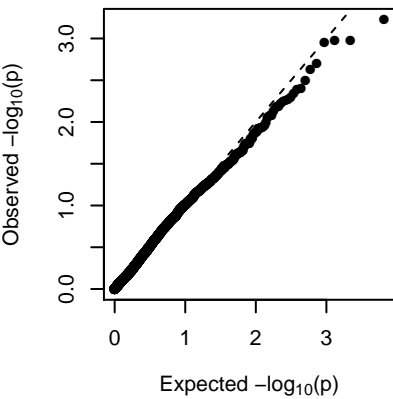
MEpink (additive)
